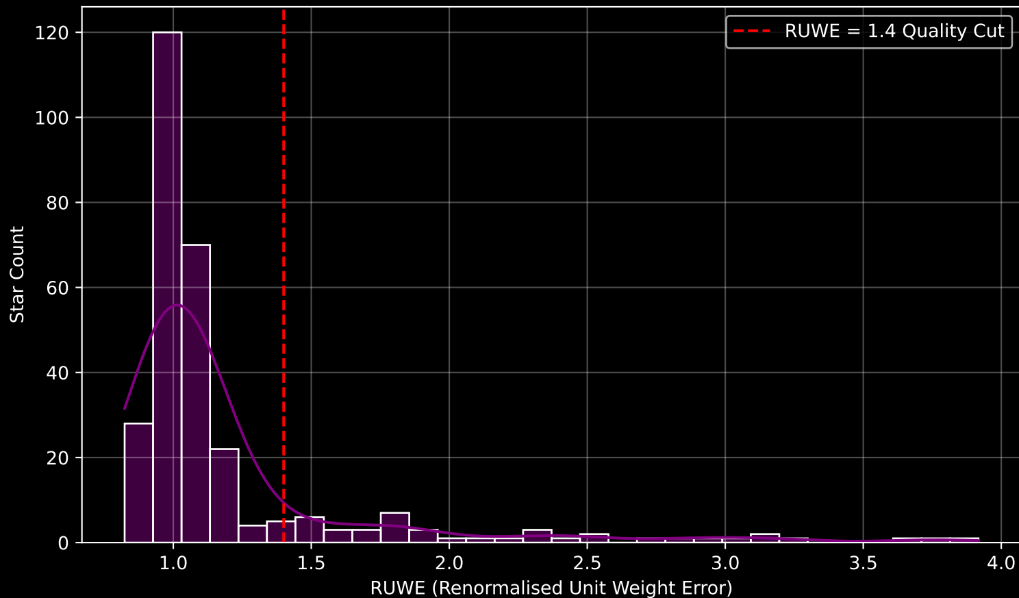
GALAH DR4 Field [132] RUWE Distribution (n= 290)
