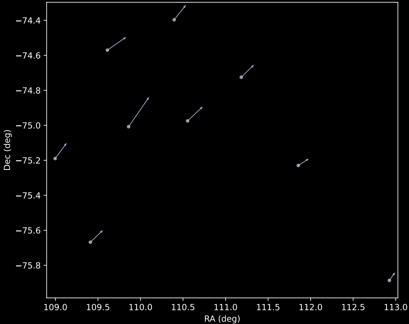
GALAH DR4 Cluster 1 Proper Motion Vectors (n=9)
