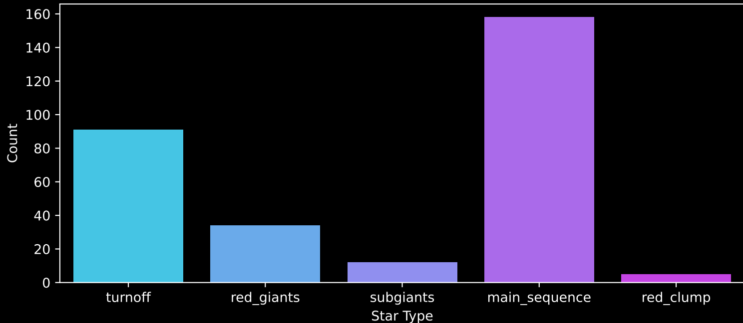
GALAH DR4 Field: [132] Count plot of Star Type
